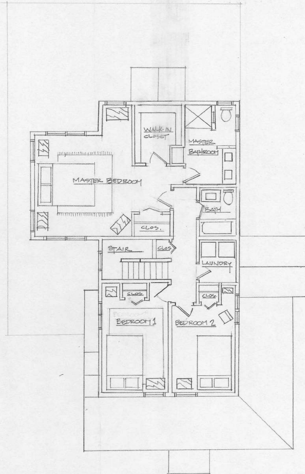
SECOND FLOOR PLAN \frac{1}{8}'' = 1'-0''
